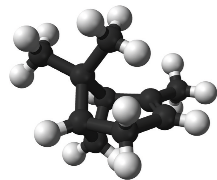
„Stone pine scent“ Structural formula C 10 H 16
